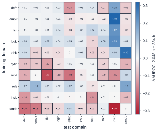
Fig. 3: The cost of a wider code, cell by cell: the change in cross-domain AUROC as the sign-RP ternary code grows from 384 to 2,048 bits (red is fidelity lost; off-diagonal cells losing more than 0.05 are outlined). The diagonal is flat to slightly positive while the transfer losses concentrate in the rows already weakest at 384 bits, so the extra capacity sharpens domain-specific boundaries rather than helping them travel (Sec. V-C).
